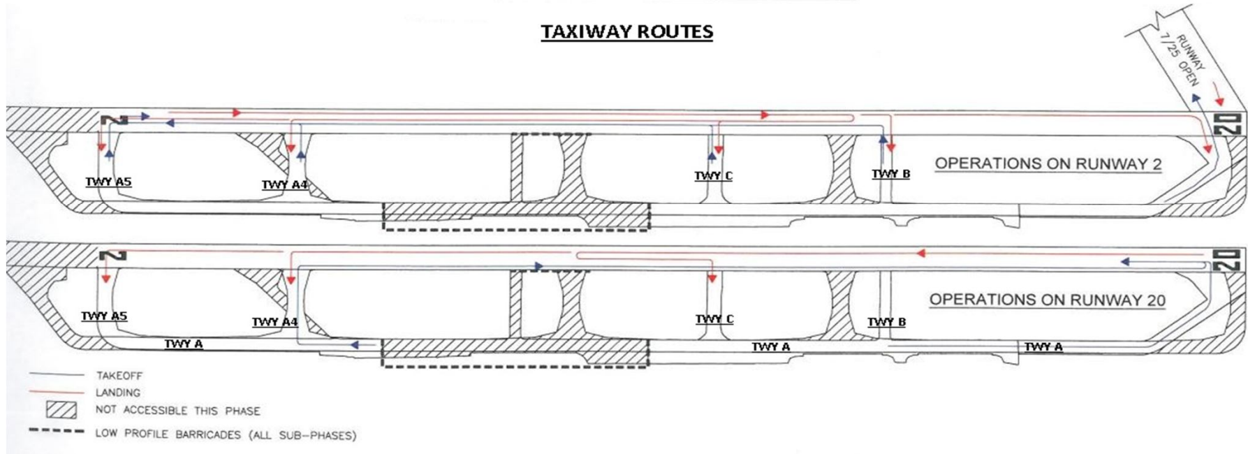
CONSTRUCTION PHASING PLAN - PHASE "2"
